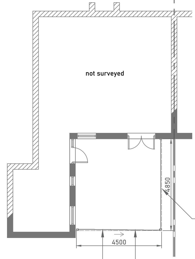
FLOOR PLAN
