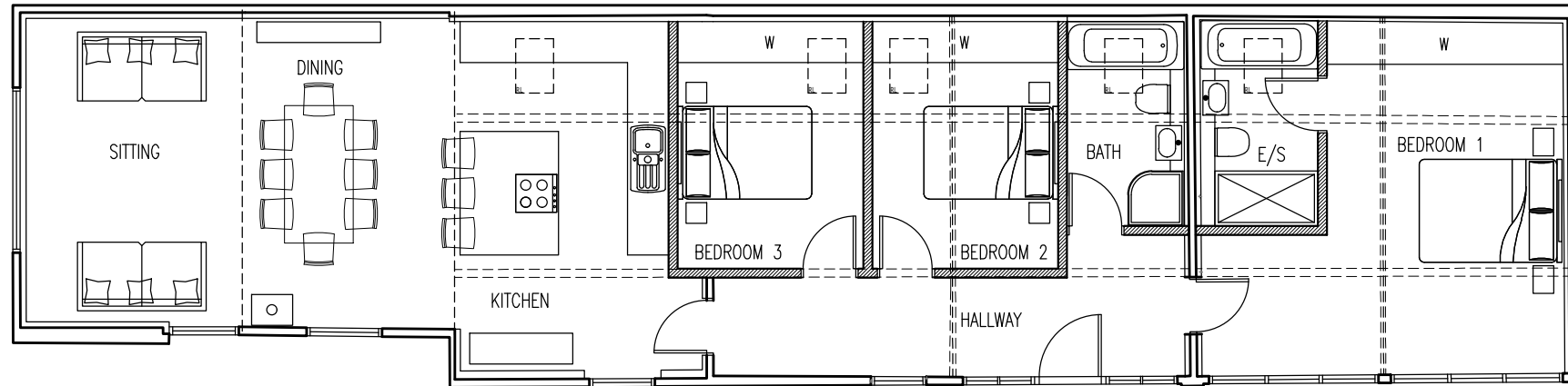
PROPOSED FLOOR PLAN
