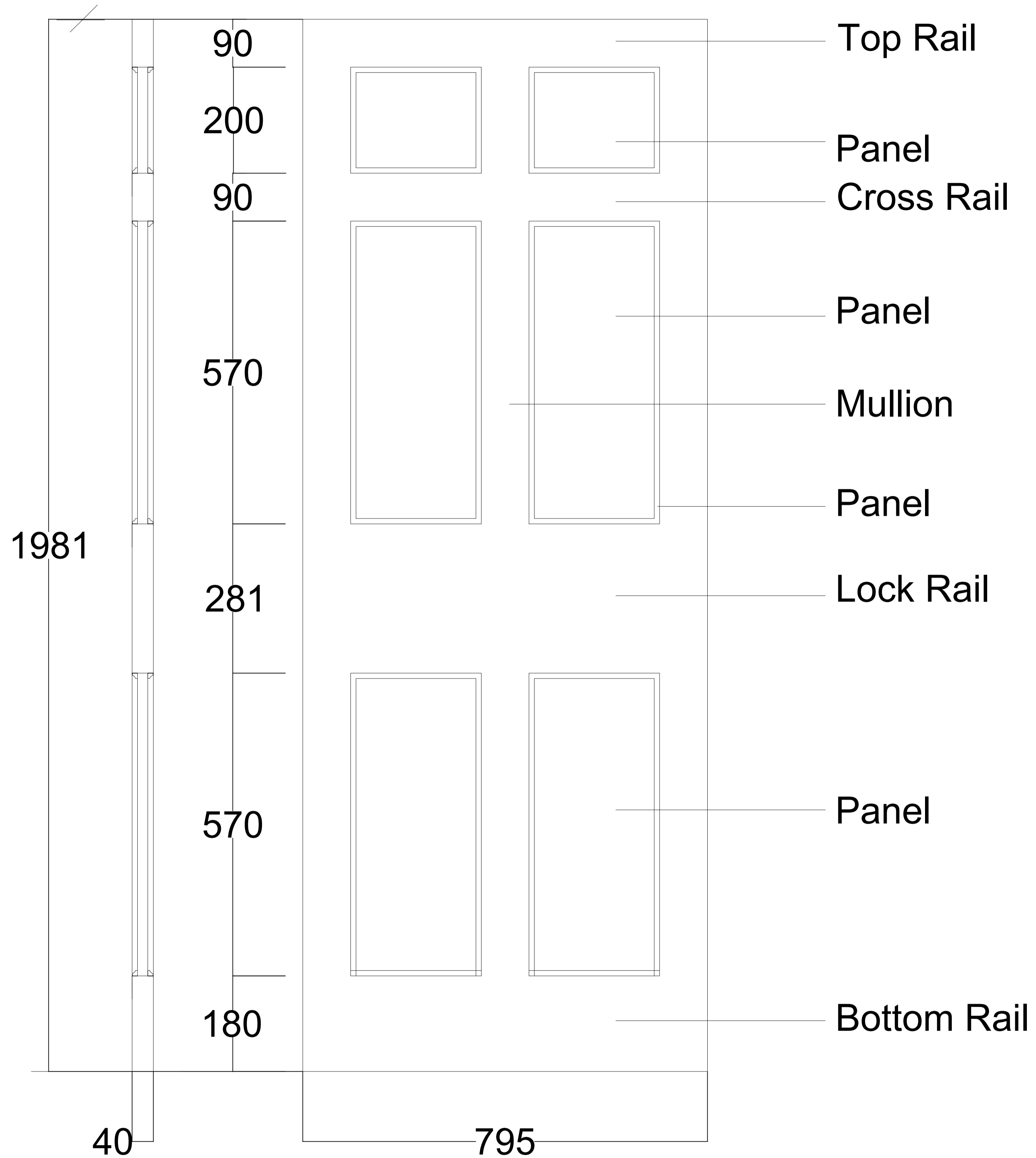
Internal Door Elevation/ Section 40mm thick pine timber door to receive paint finish
