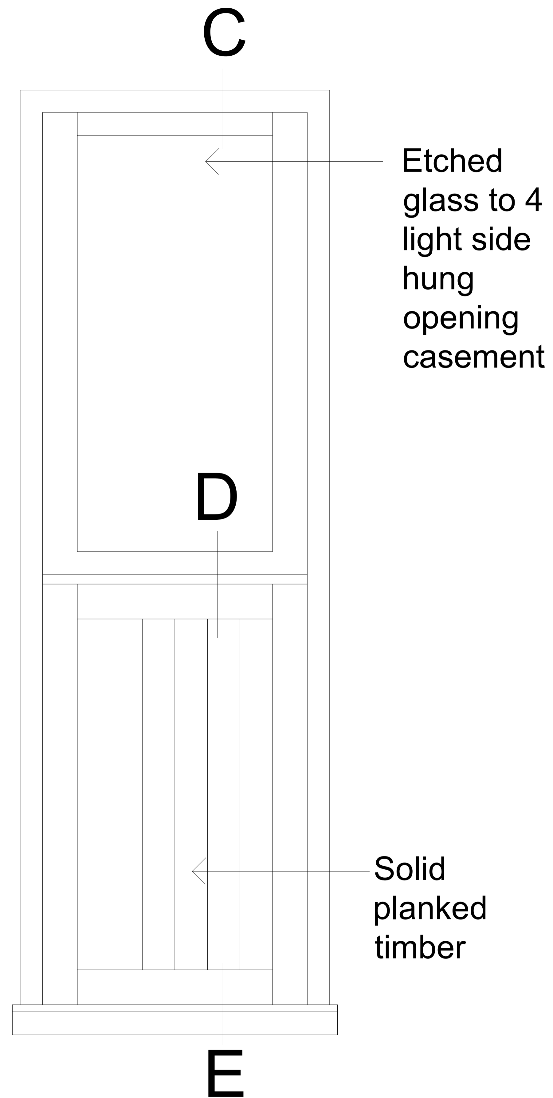
Window Elevation House - Timber painted to match existing
