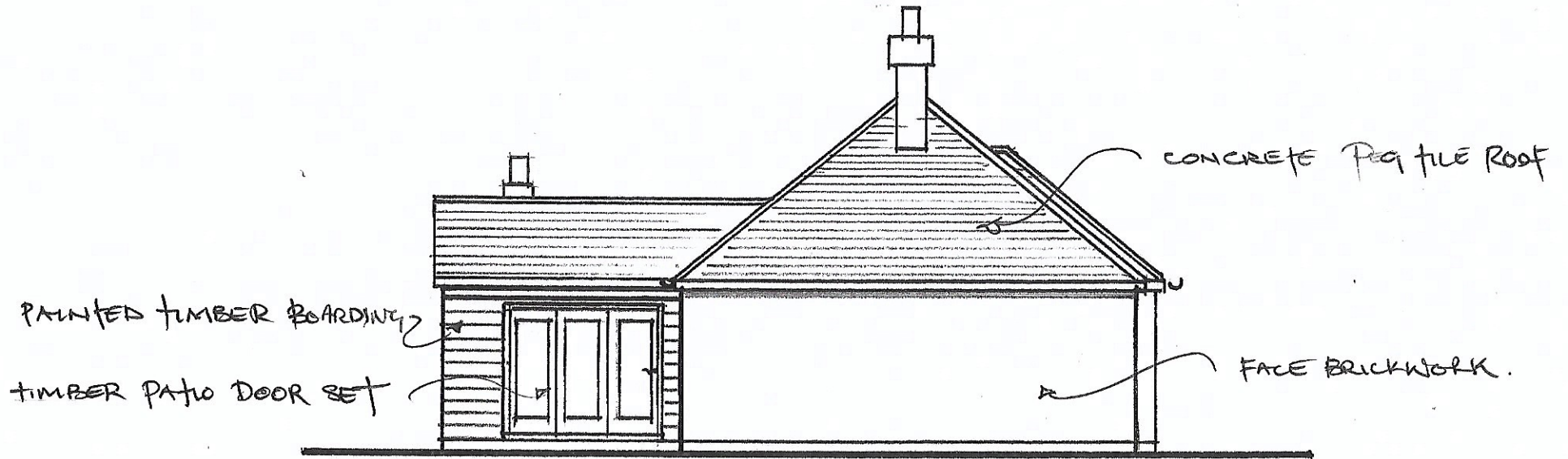
SIDE ELEVATION AS EXISTING 1:100/NORTH WEST
