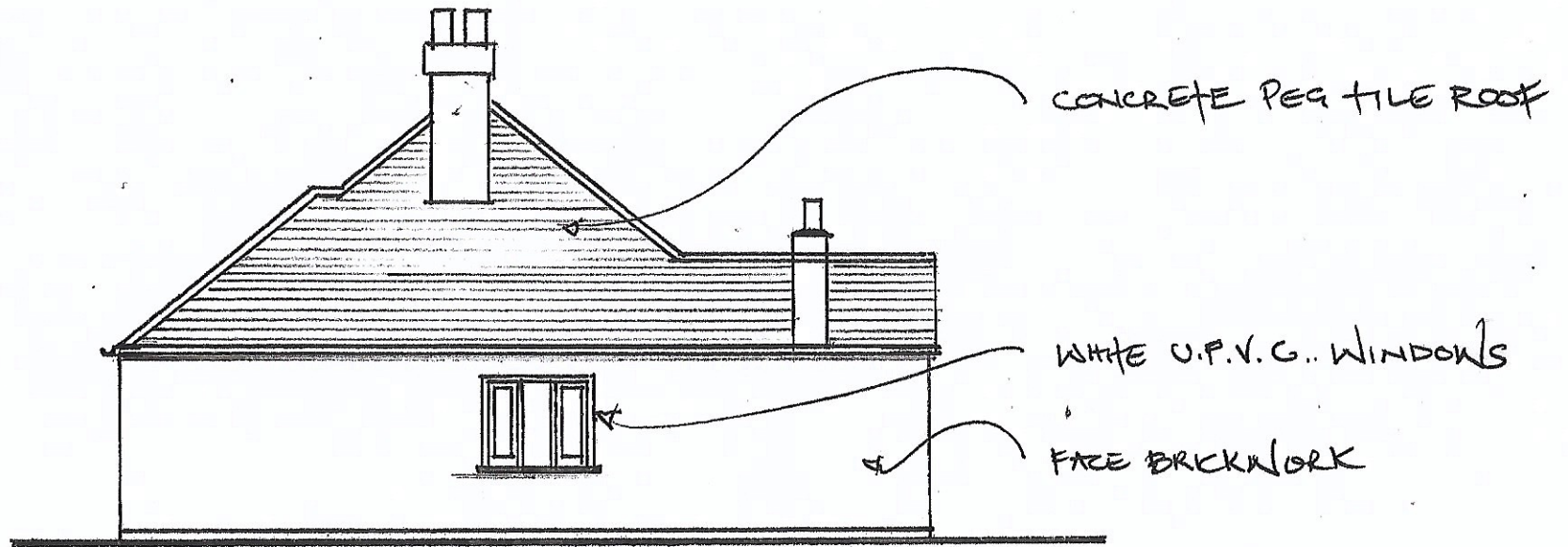
SIDE ELEVATION AS EXISTING 1:100 / SOUTH EAST
