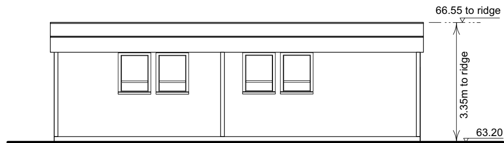
SIDE/WEST ELEVATION
