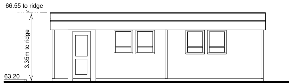
SIDE/EAST ELEVATION
