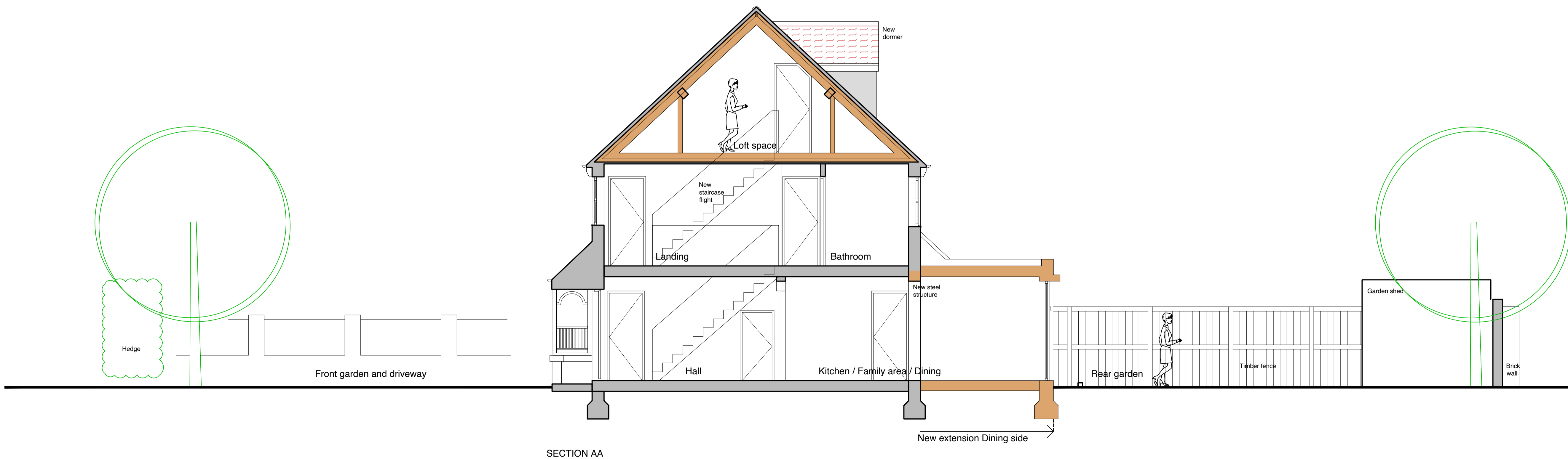
SECTION AA
