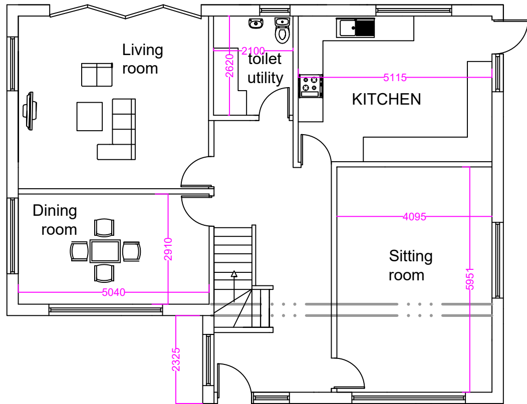
PROPOSED GROUND FLOOR PLANS
