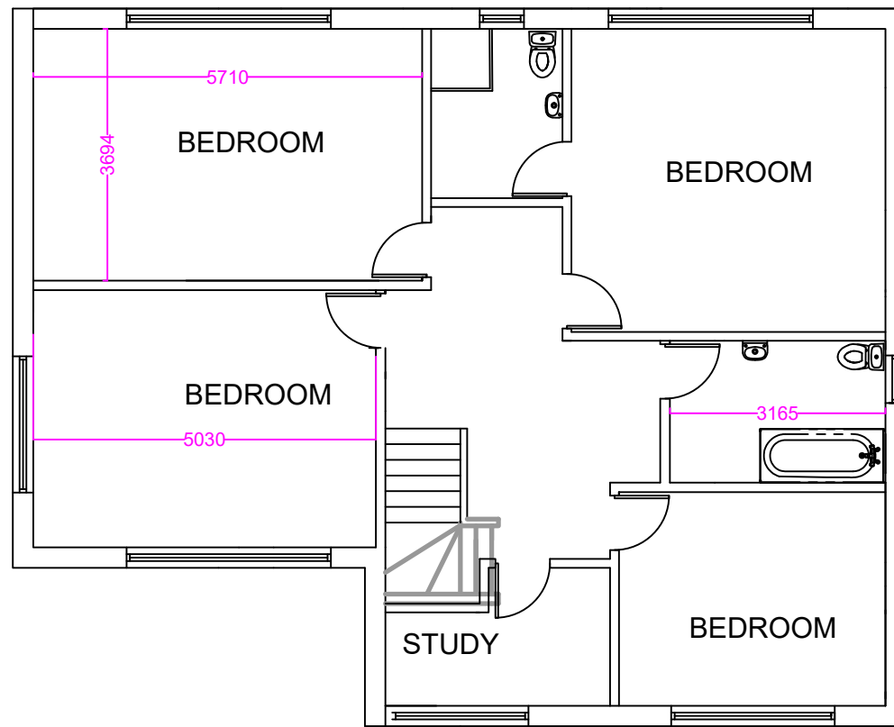
PROPOSED 1ST FLOOR PLANS
