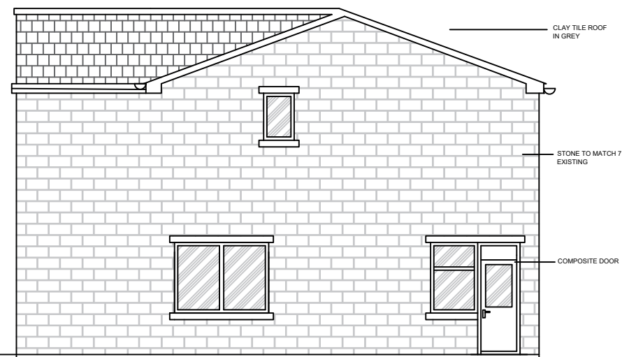
PROPOSED RIGHT SIDE ELEVATION
