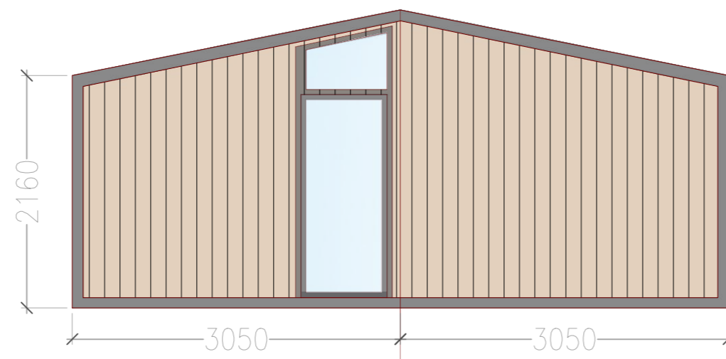
Front elevation
