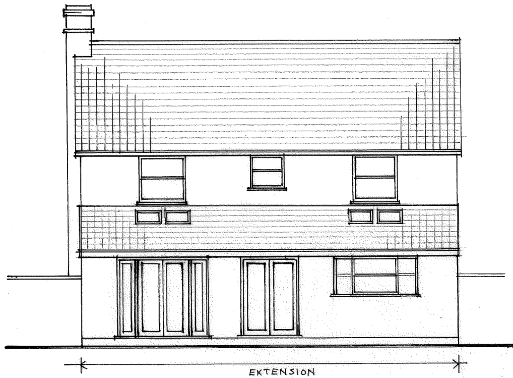
BACK · EAST · ELEVATION
