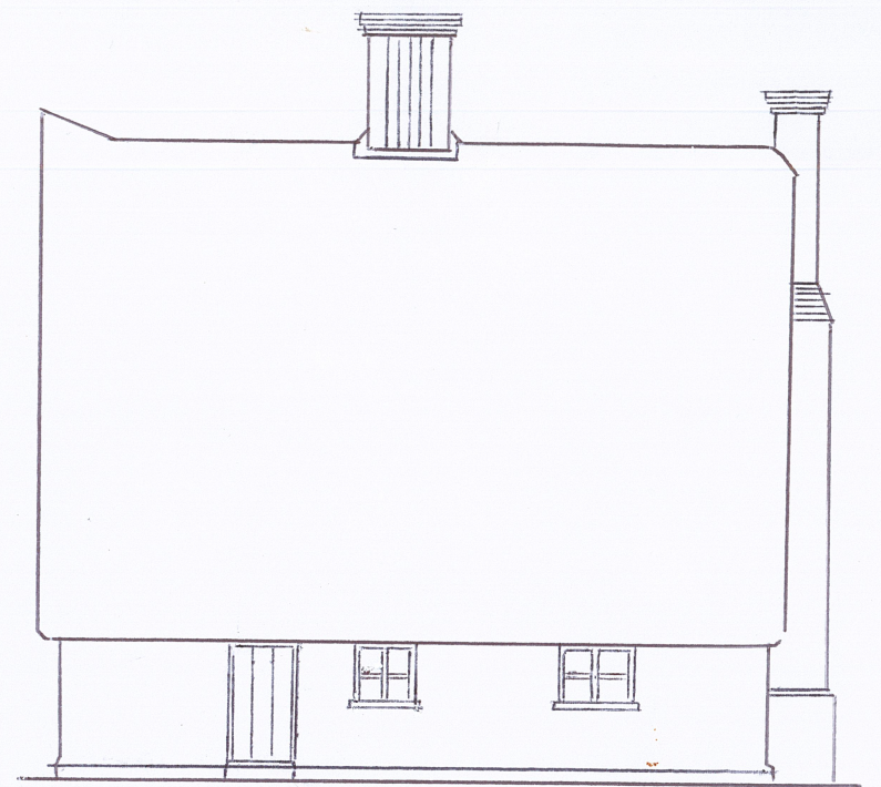
REAR ELEVATION - NORTH WEST
