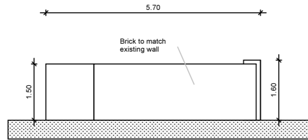
Proposed Garden Wall South West Facing Front Elevation
