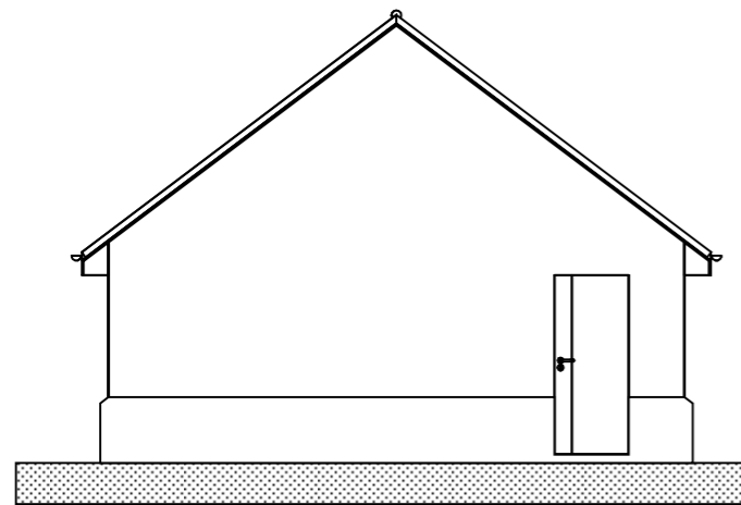
Proposed Garage North West Facing Side Elevation
