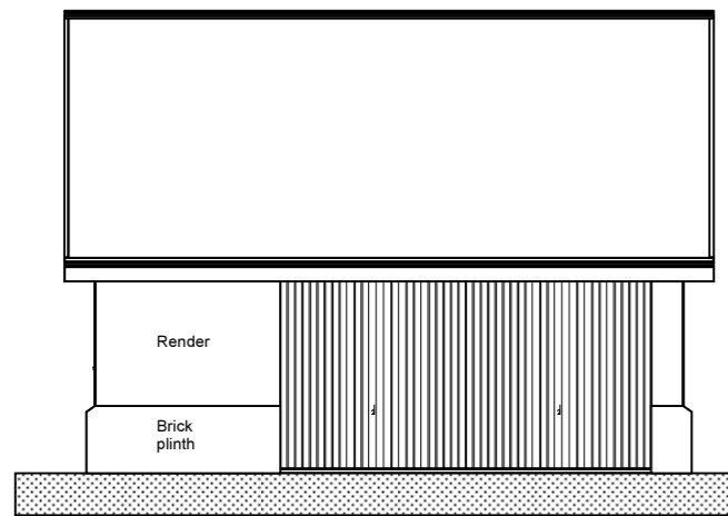
Proposed Garage South West Facing Front Elevation
