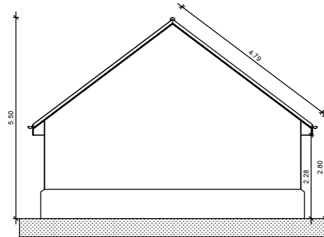
Proposed Garage South East Facing Side Elevation
