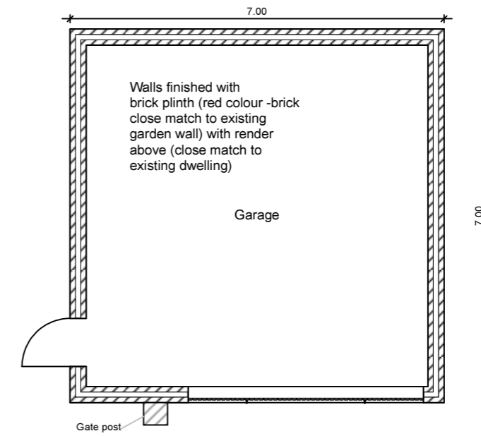
Proposed Garage Floor Plan
