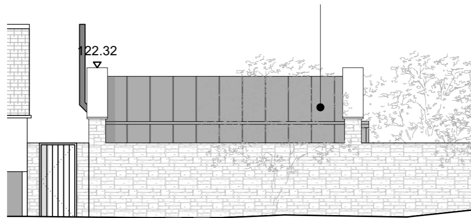
South-east facing elevation and roof slope clad in zinc
