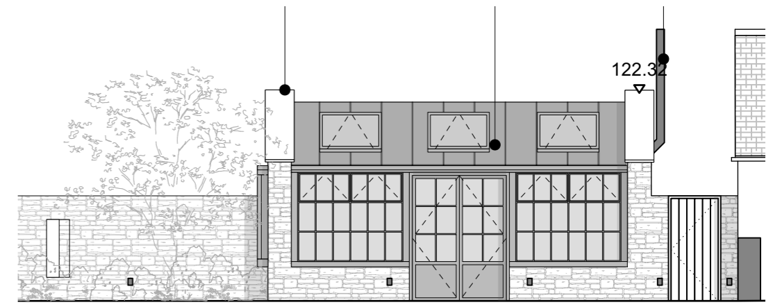
North-west facing elevation, glazed as per approved design, with revised roof slope clad in zinc with 3no rooflights flush with roof slope
