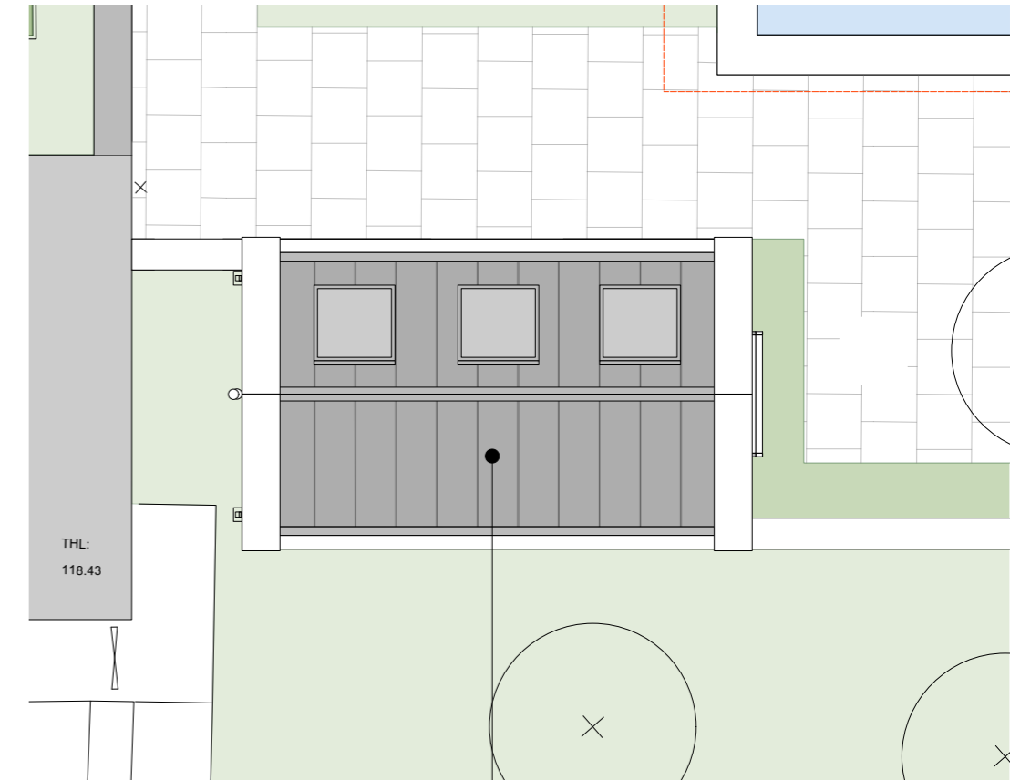
Roof plan of Art Studio with revised material palette of zinc-cladding with 3no rooflights
