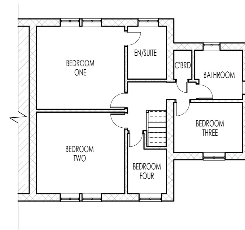
FIRST FLOOR
