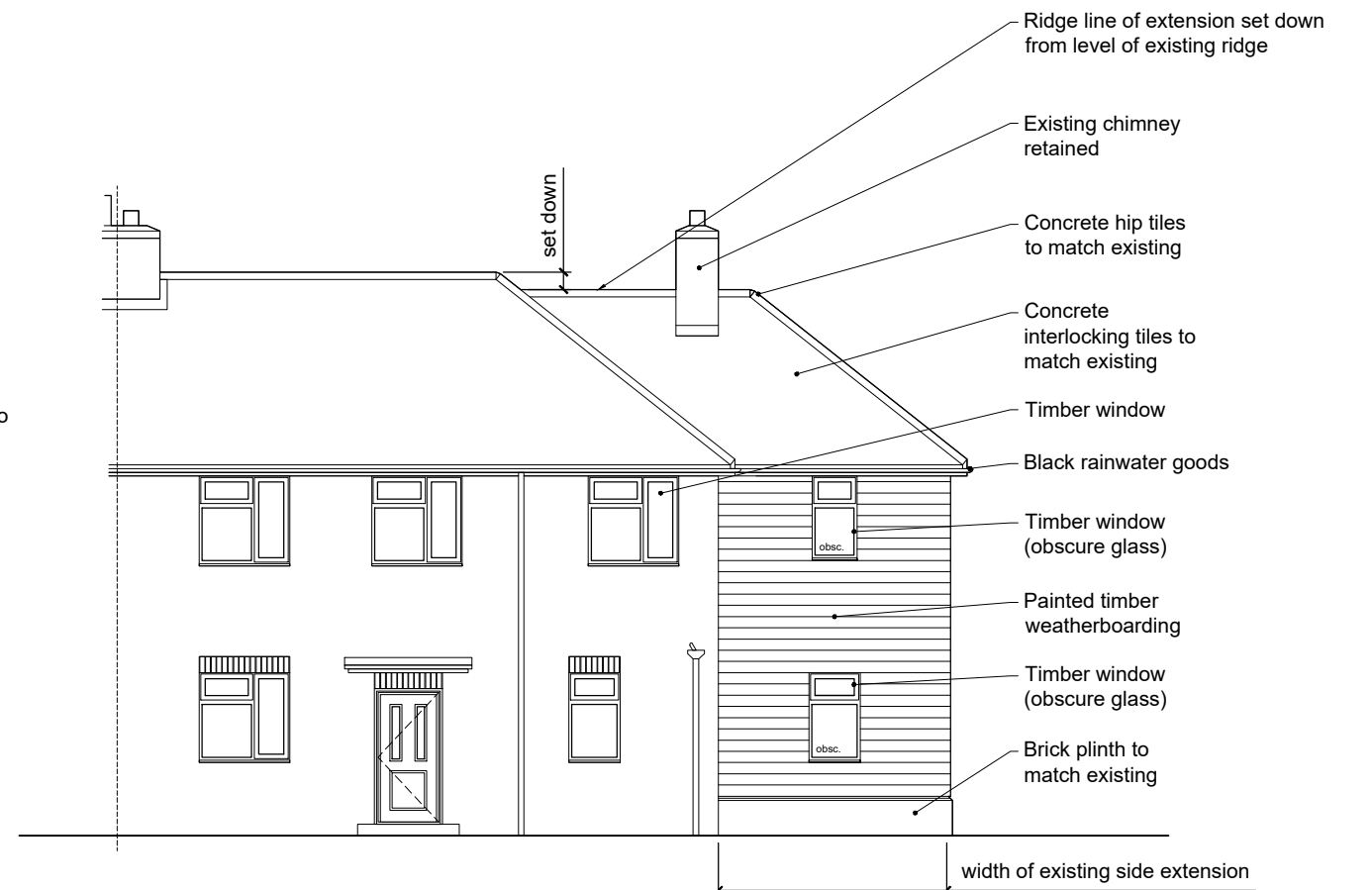
PROPOSED SW ELEVATION
