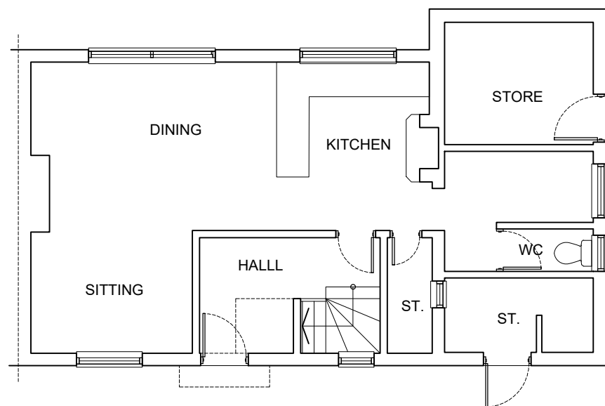
EXISTING GROUND FLOOR
