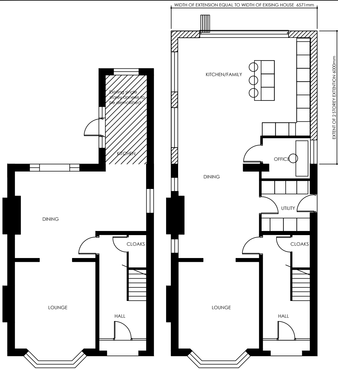
EXISTING GROUND FLOOR SCALE 1:100
