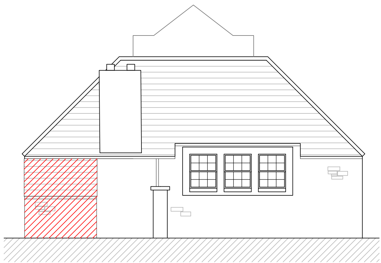
South Elevation 1:100
