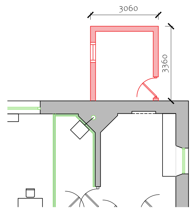
Floor Plan of Shed 1:100
