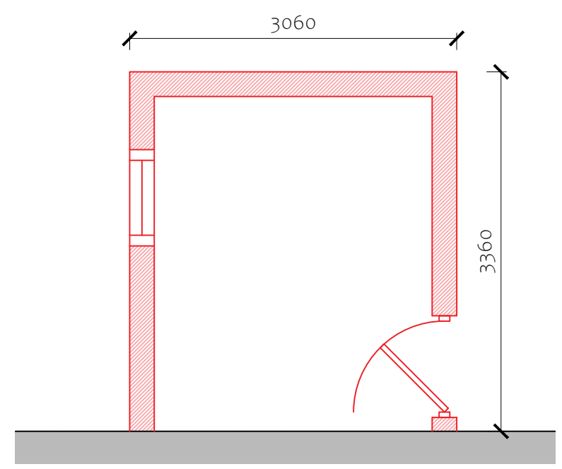
Floor Plan of Shed 1:50
