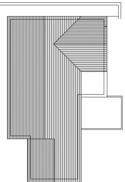
ROOF LAYOUT 1:200
