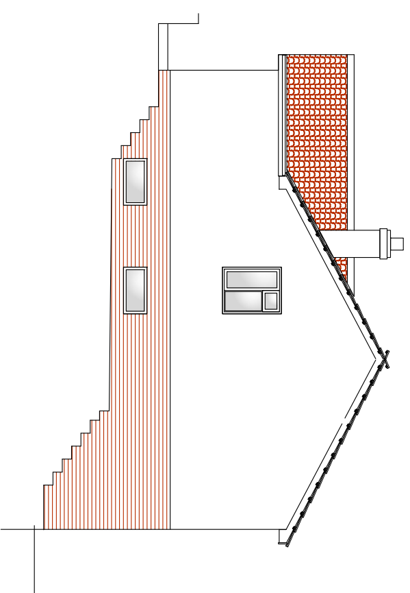
EAST ELEVATION
