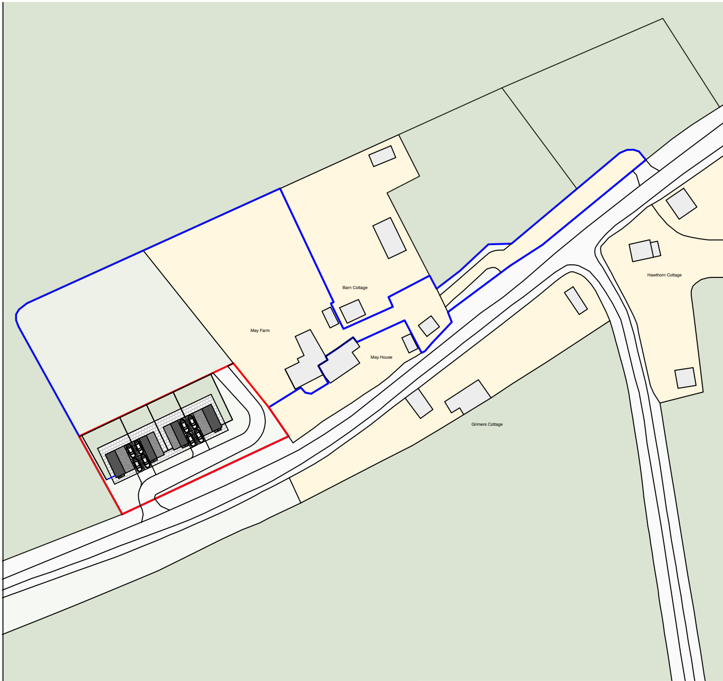
Proposed Location Plan - Scale 1:1250 @ A4
