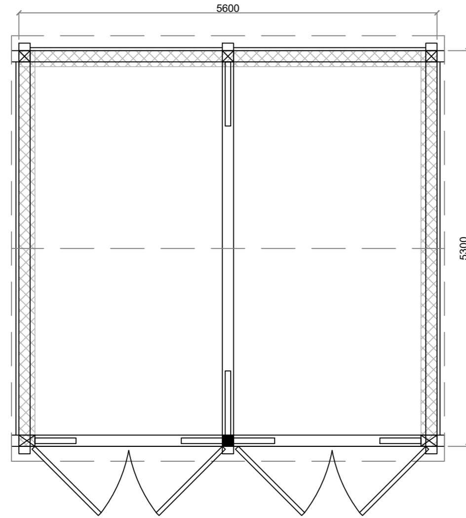
Floor / Frame Plan
