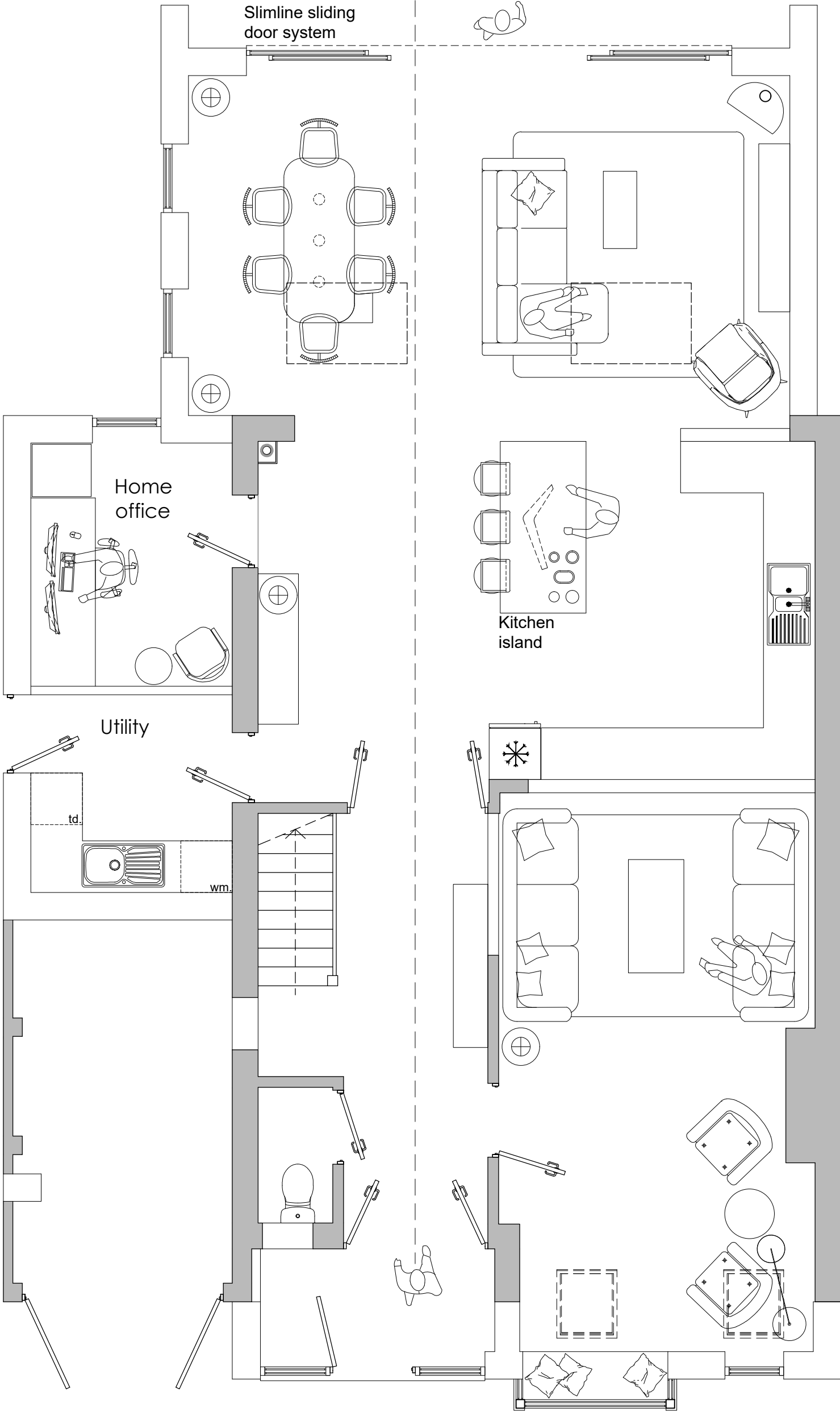
Proposed Ground Floor Plan scale 1:50@A3
