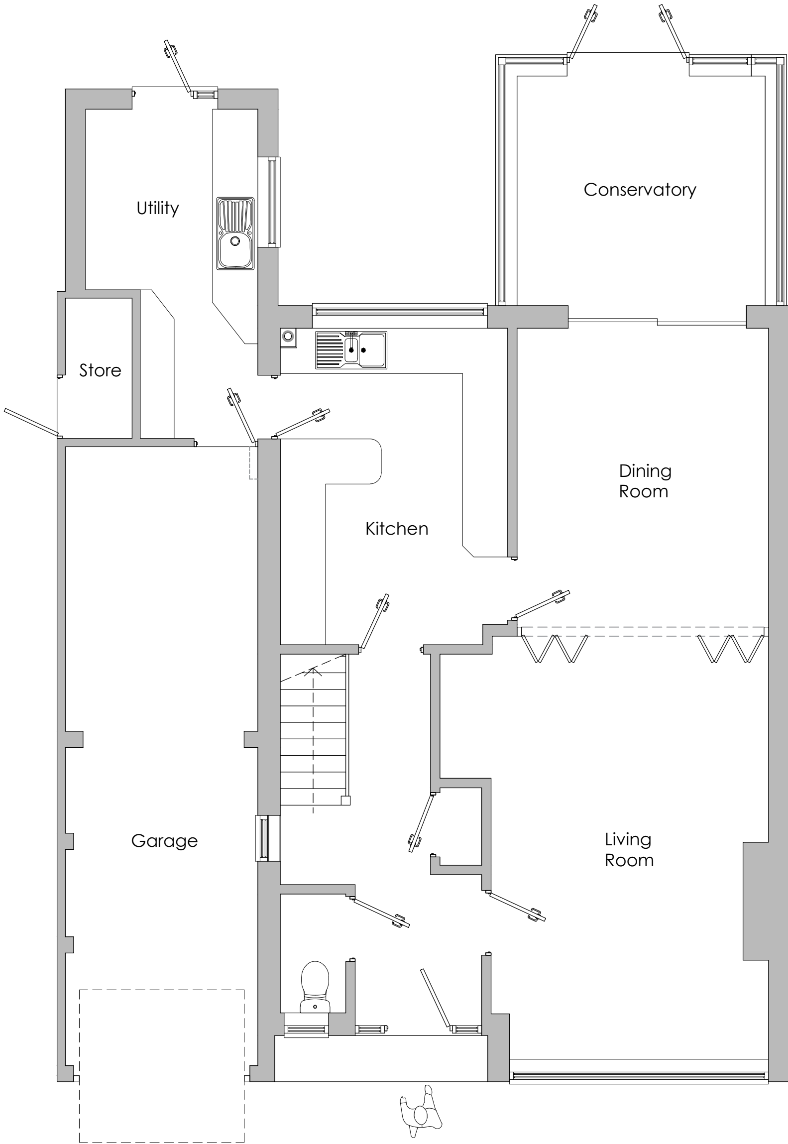
Existing Ground Floor Plan scale 1:50@A3
