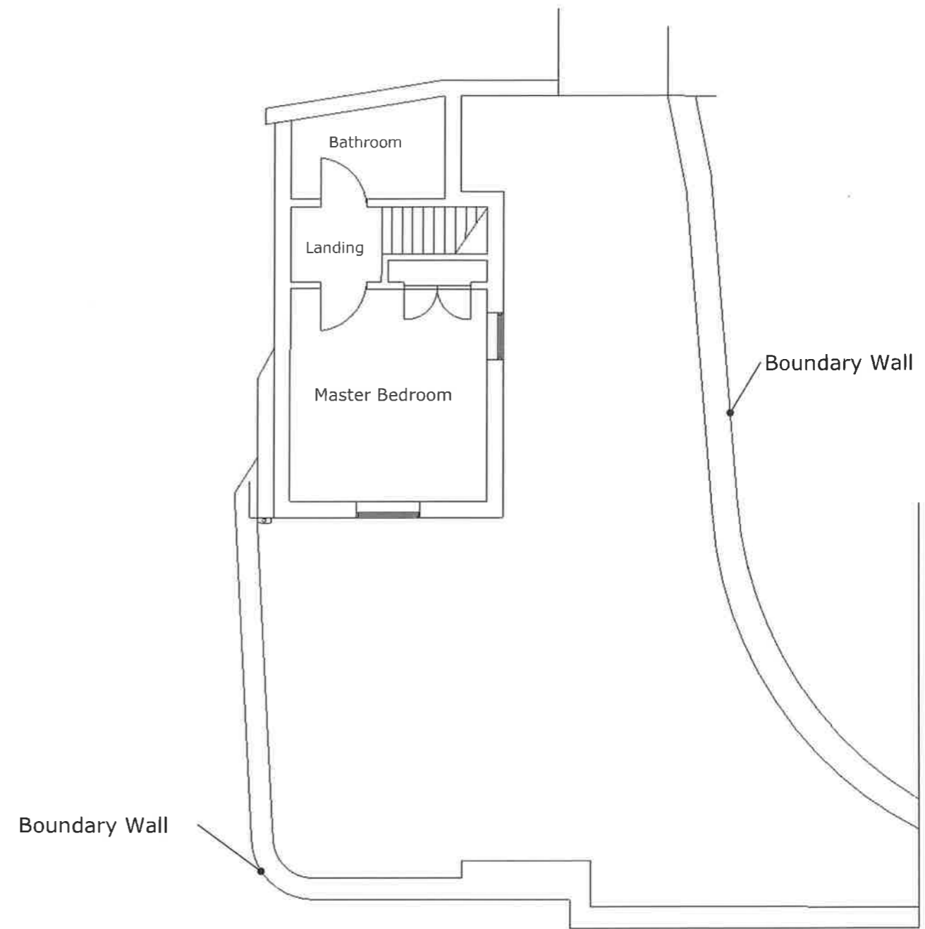
EXISTING FIRST FLOOR LAYOUT
