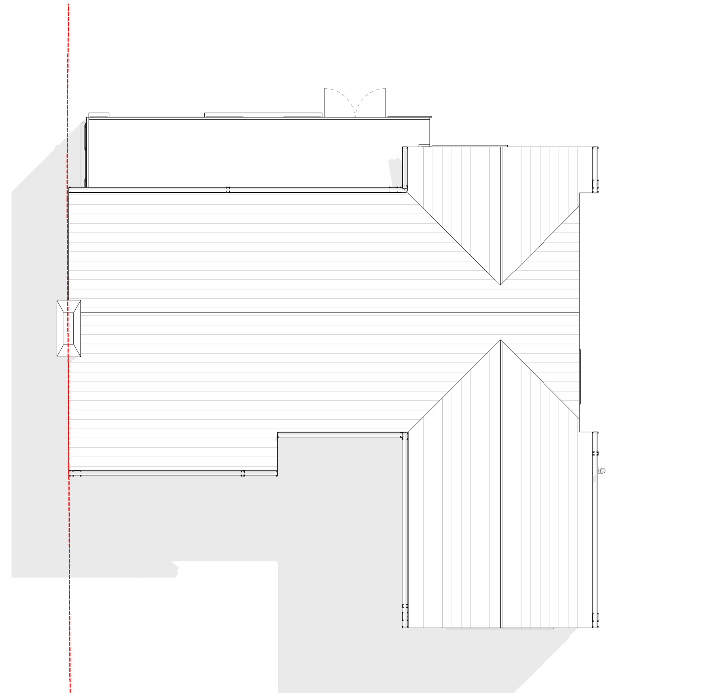
Existing Roof Plan 1 : 50
