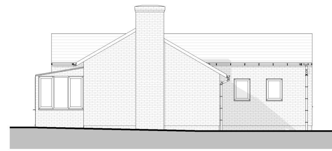
4 Existing Left Side Elevation 1 : 100
