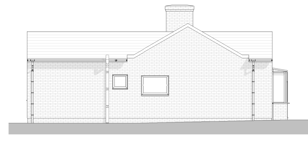
3 Existing Right Side Elevation 1 : 100
