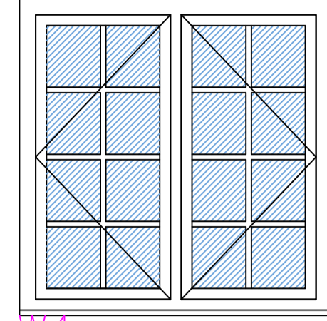
W4 1245 x 1220 Window to incorporate slimline double glazing.
