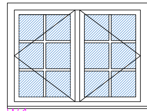
W1 1245 x 960 Window to incorporate slimline double glazing.
