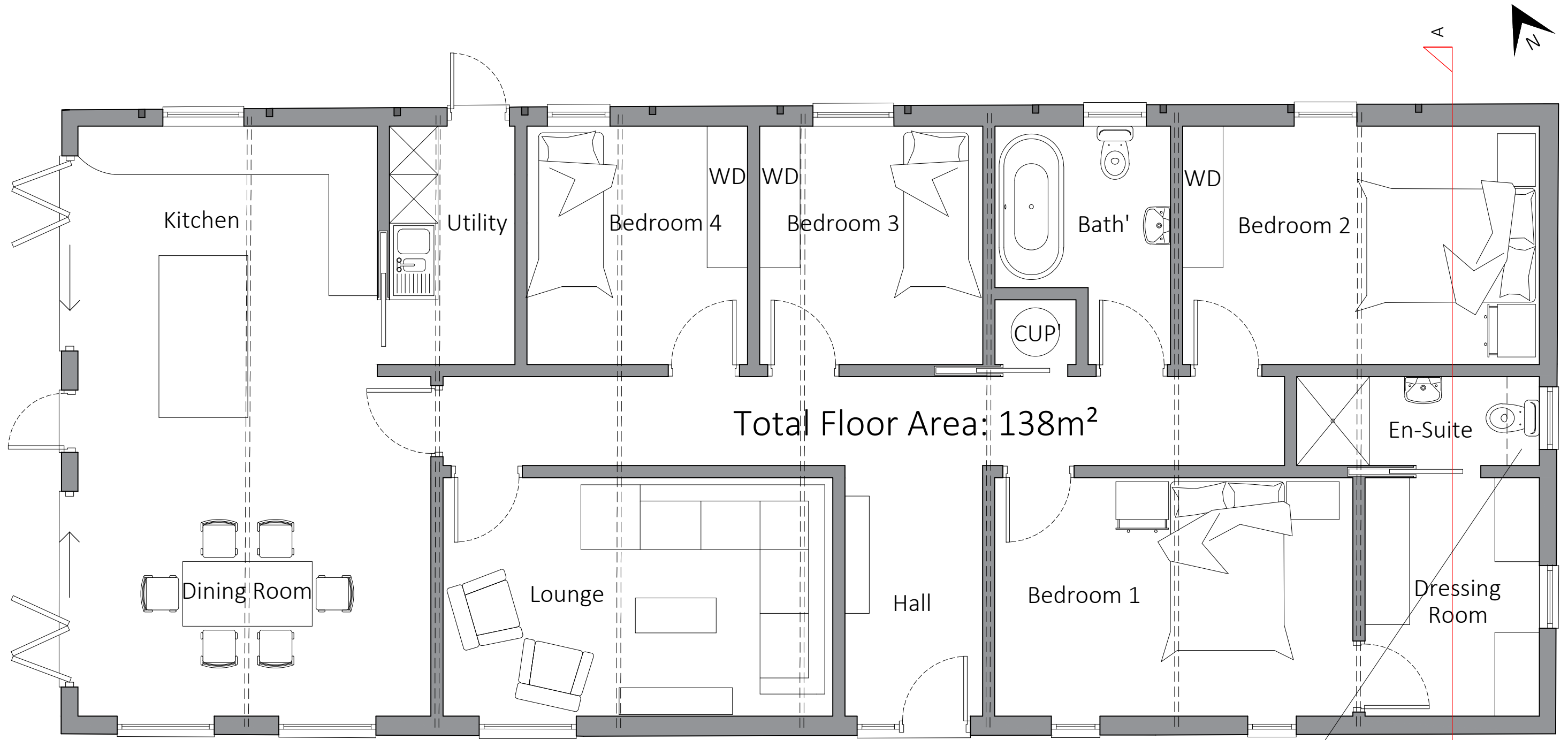
Proposed - Ground Floor Plan 1:50 @ A3
