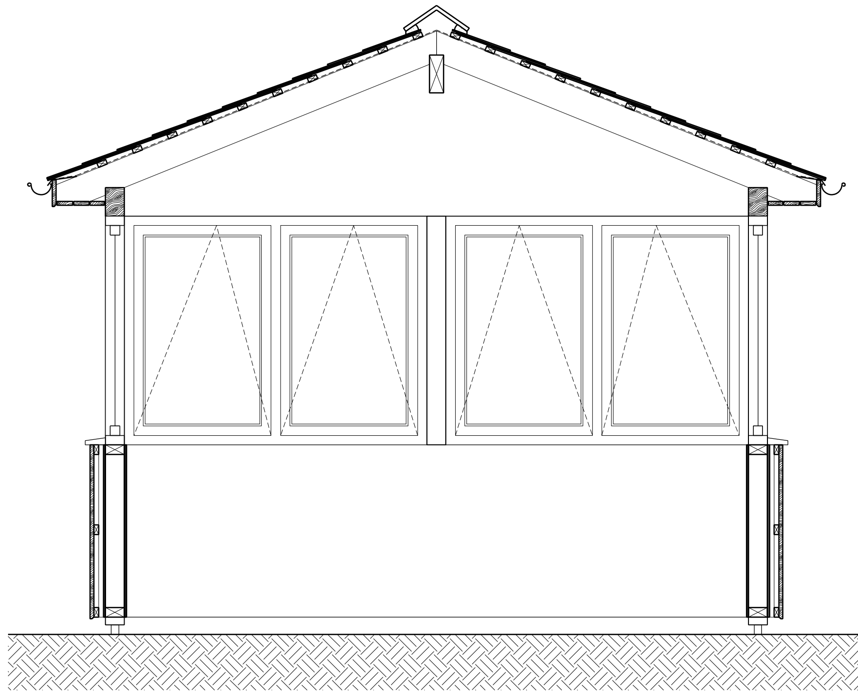
Section B-B
