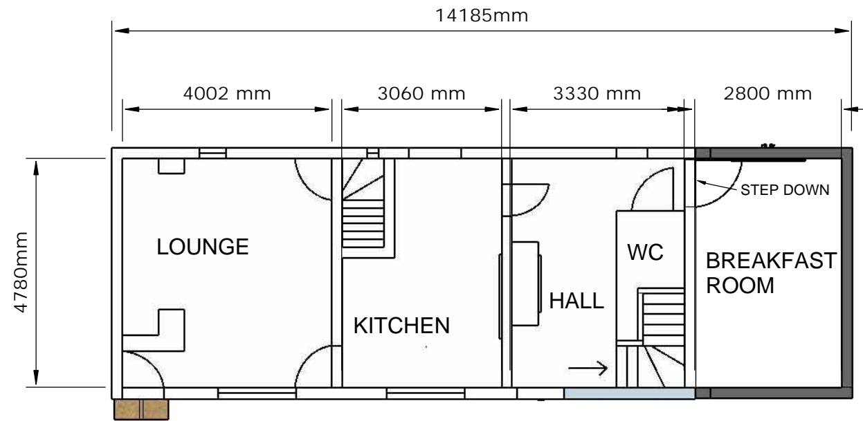
GROUND FLOOR
