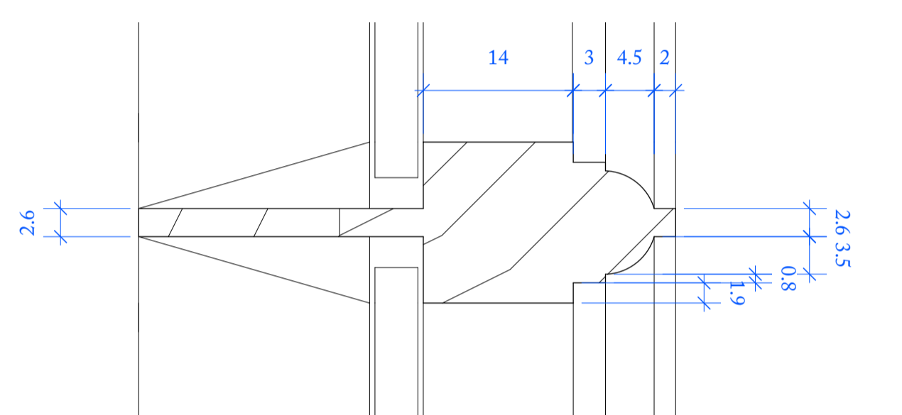
3 HISTORIC GLAZING BAR 1:1 @ A3
