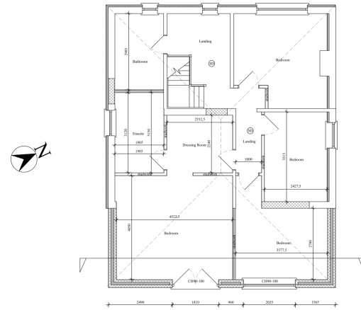
PROPOSED FIRST FLOOR PLAN 1:100
