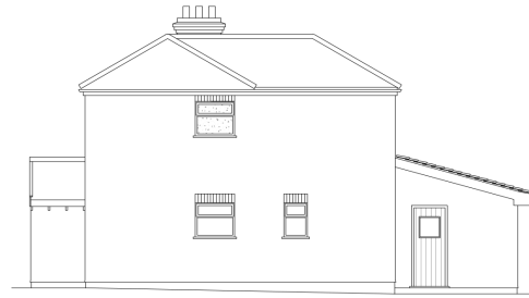
EXISTING SOUTH WEST ELEVATION, 1:100
