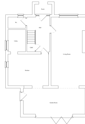
EXISTING GROUND FLOOR PLAN 1:100
