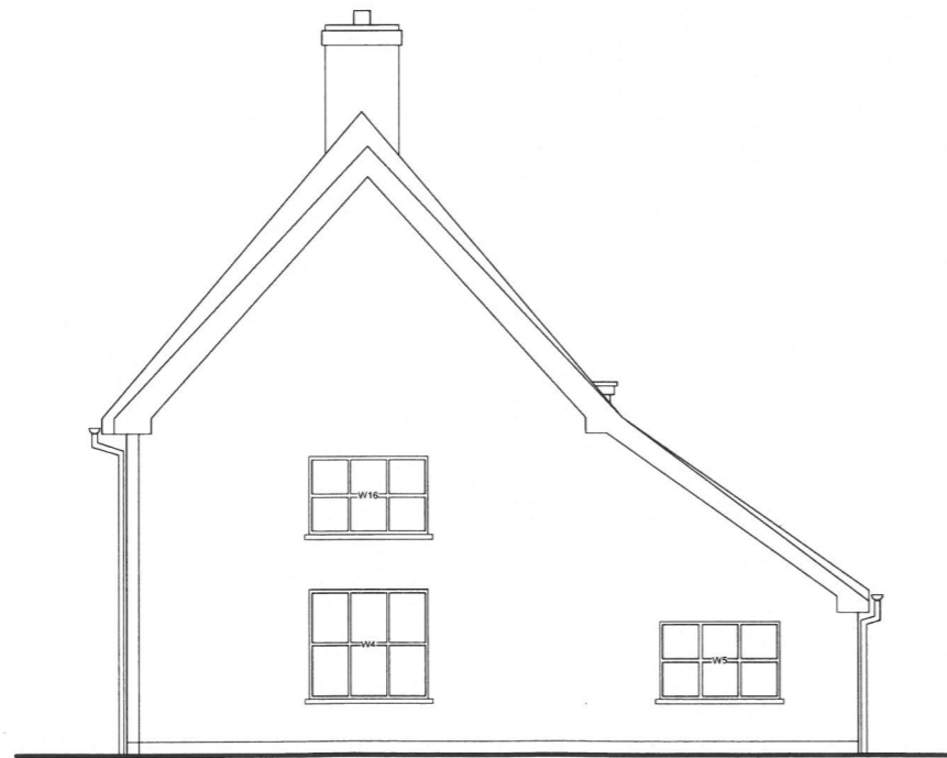
SIDE ELEVATION 1
