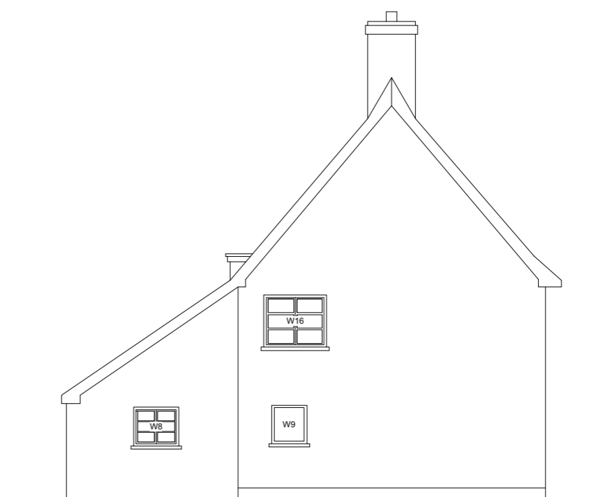
SIDE ELEVATION 2
