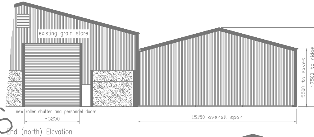
End (north) Elevation
