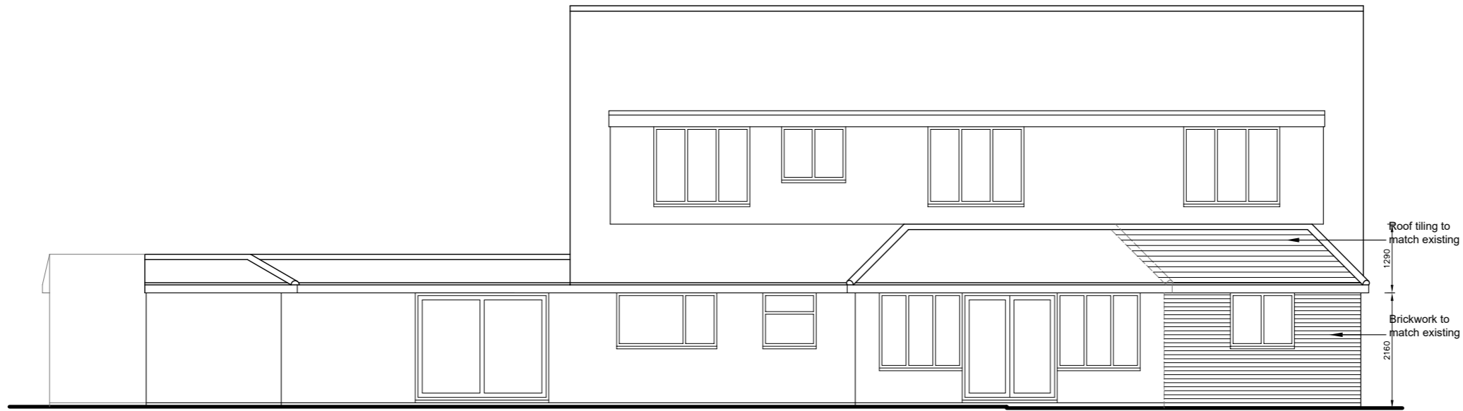
PROPOSED REAR ELEVATION 1:100
