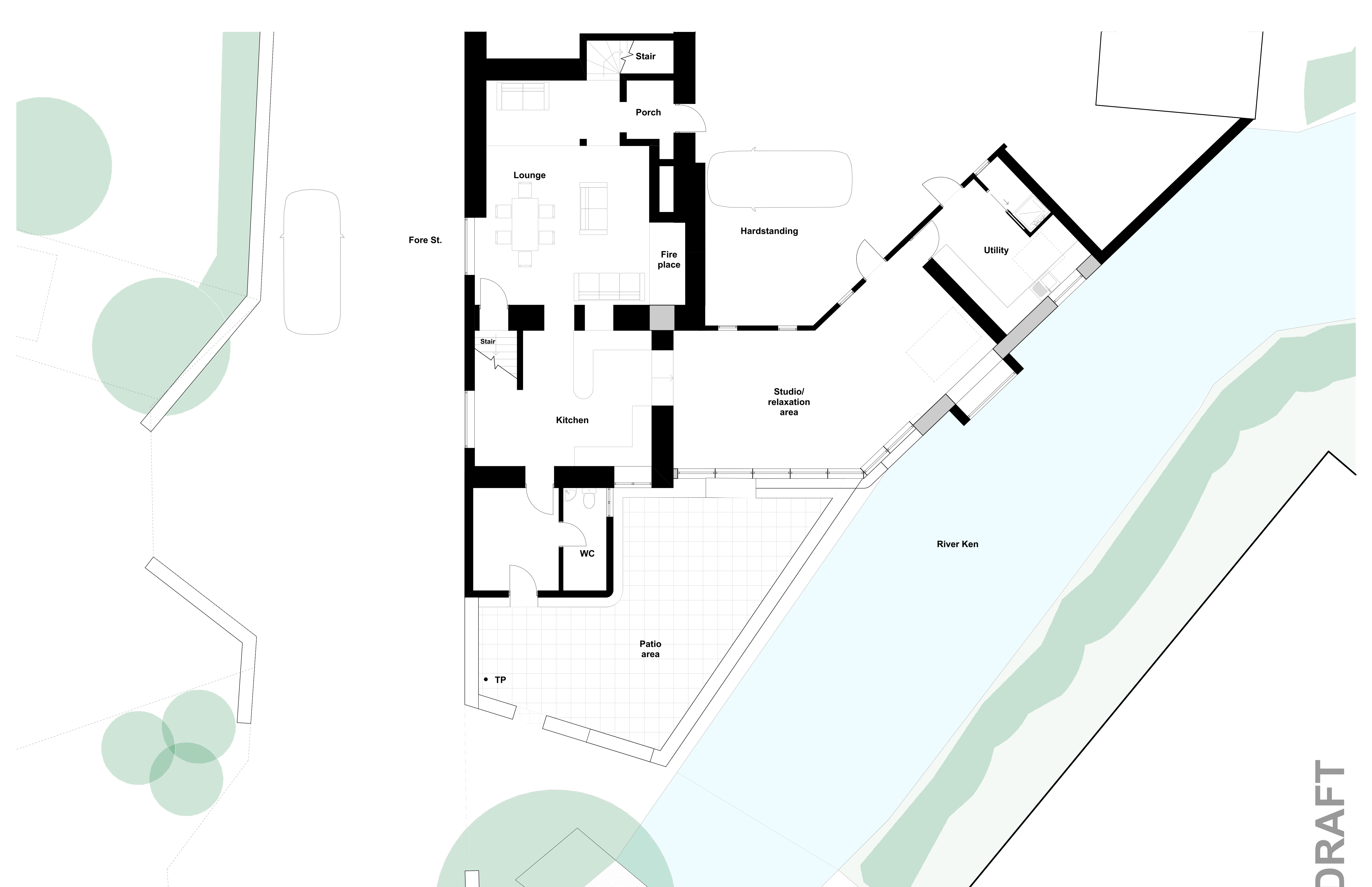
Proposed Ground Floor @ 1:50
