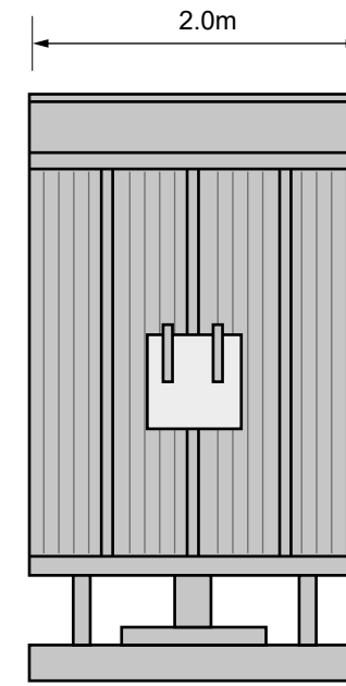
NORTHERN ELEVATION
