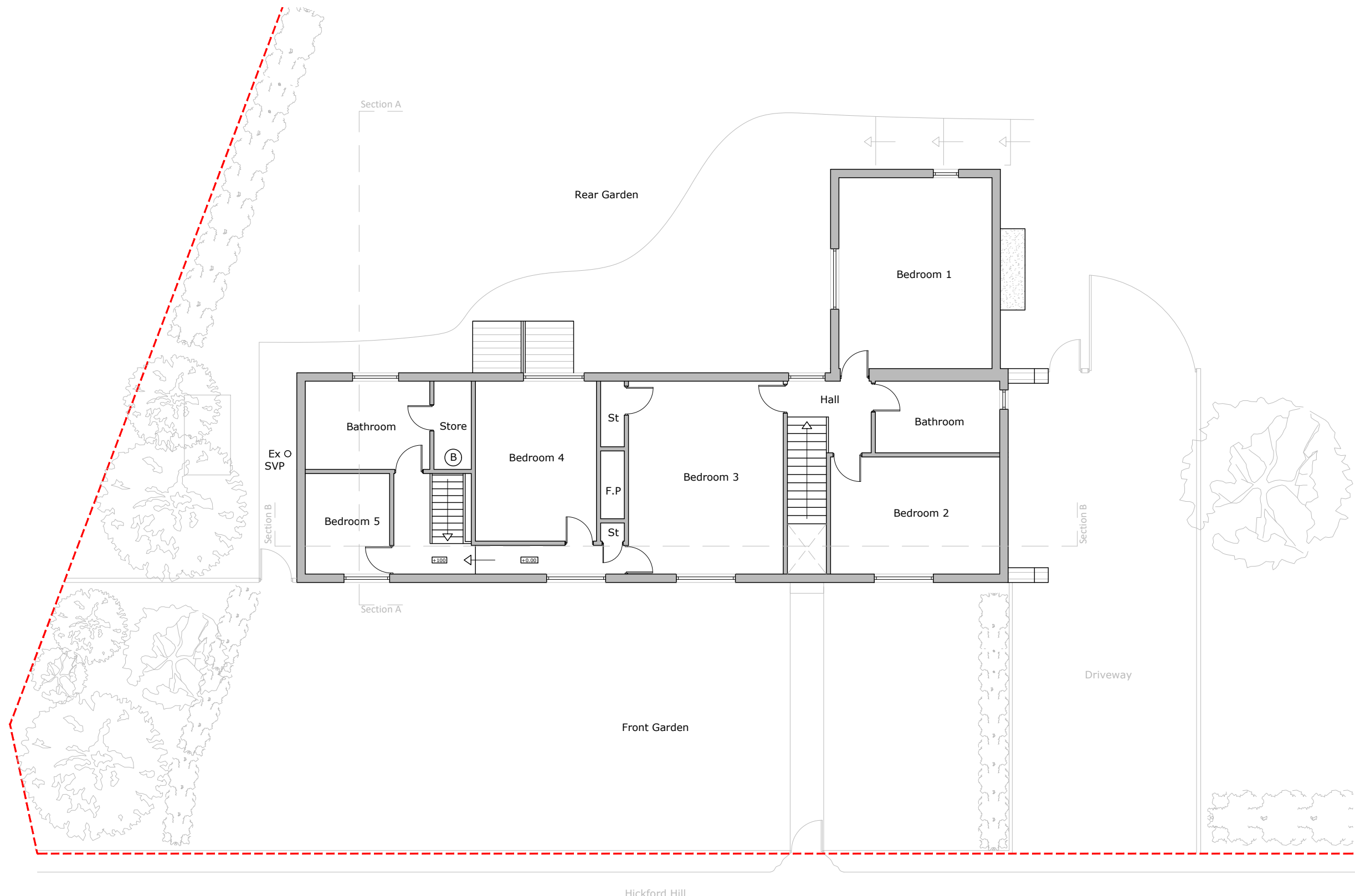
1 Existing First Floor Plan 1:100
