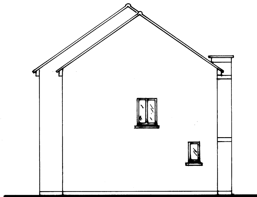
EAST ELEVATION
