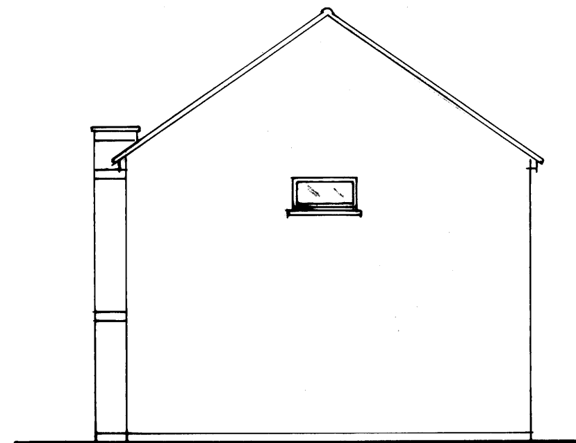
WEST ELEVATION
