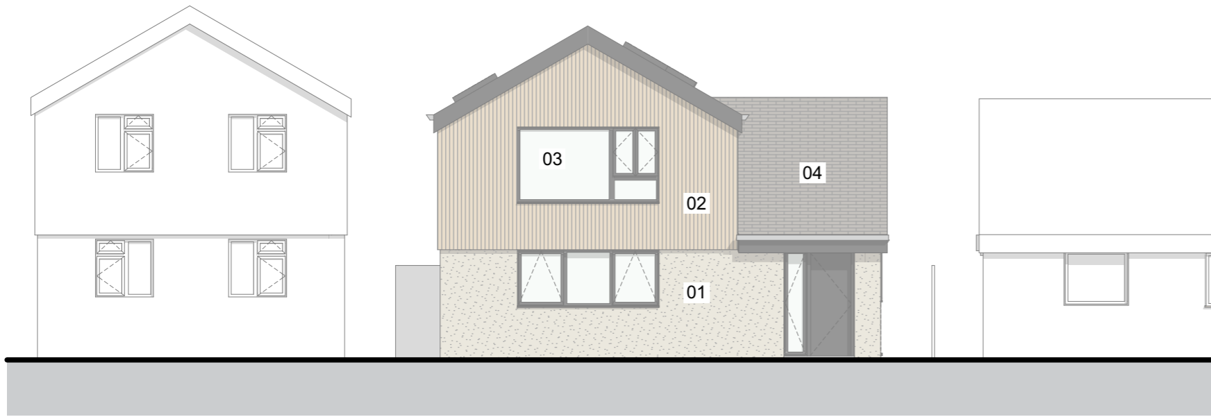
(East) Front Elevation
