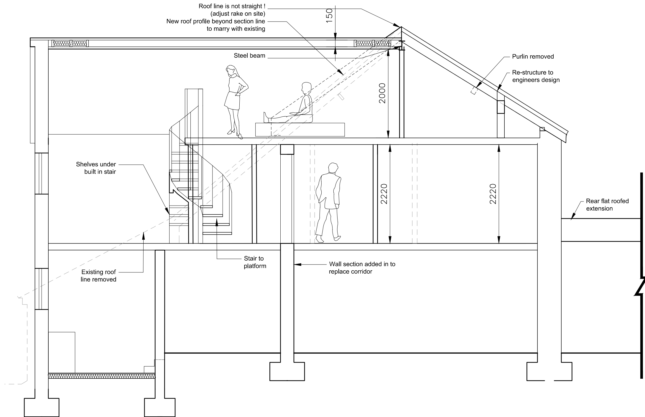
Cross section CC thro' new extension 1:50
