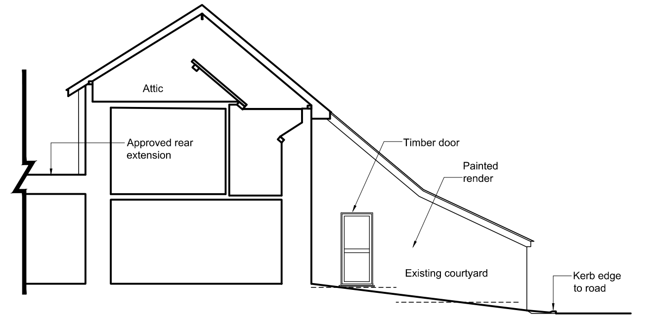
East Elevation/Section of lean to
