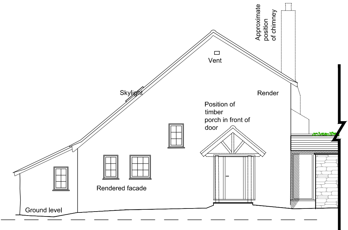
West (Entry) Elevation
