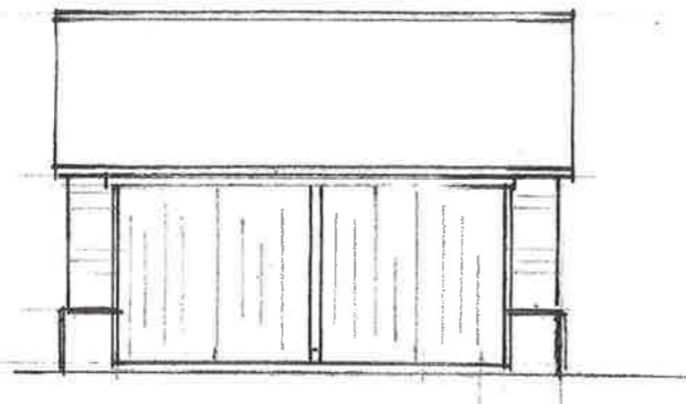
NORTH FRONT
