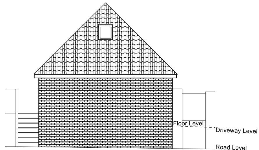
Existing Northwest Elevation
