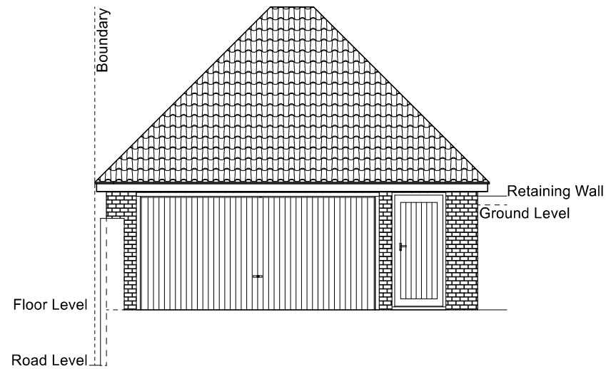
Existing Southwest Elevation
