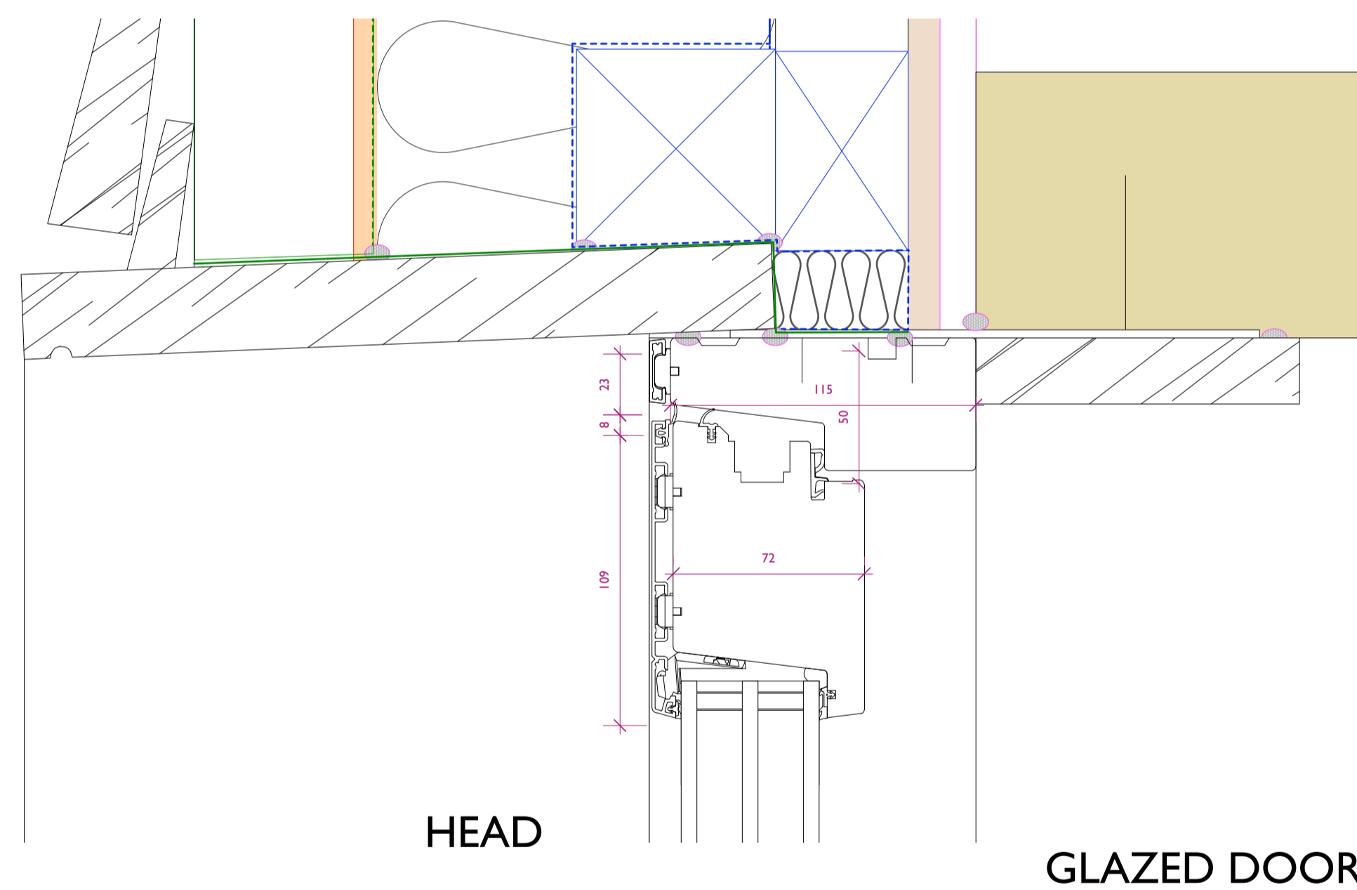
HEAD
