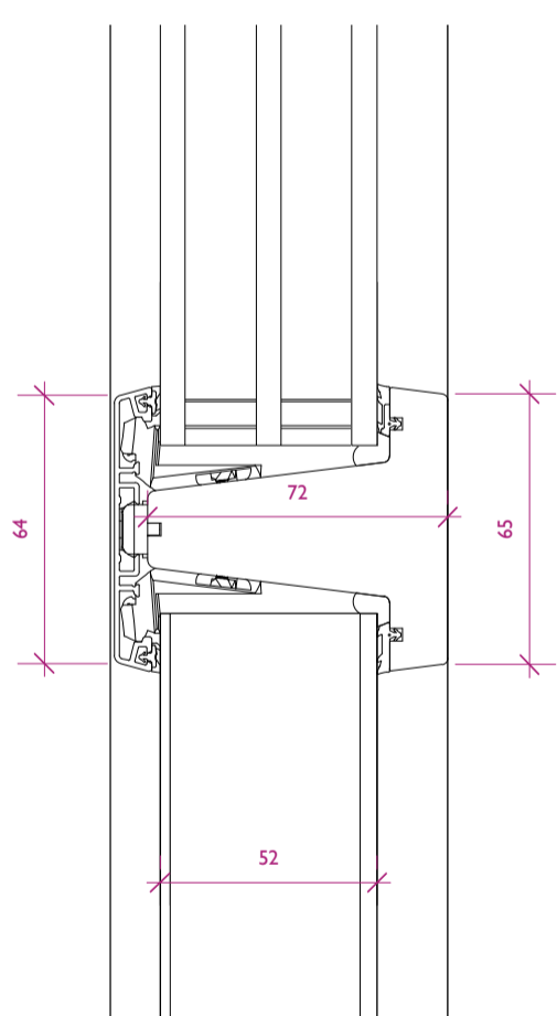
MID RAIL
