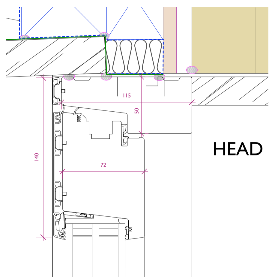
PLAN DETAILS 1:2 Scale HALF GLAZED DOOR
