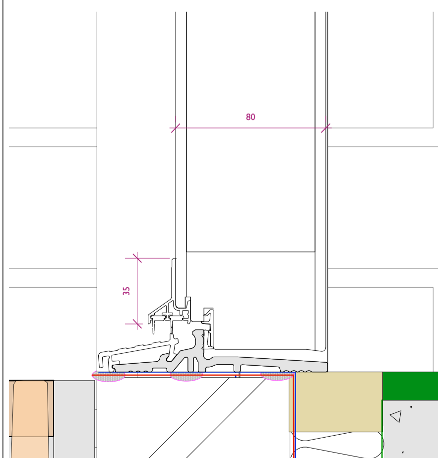
THRESHOLD
