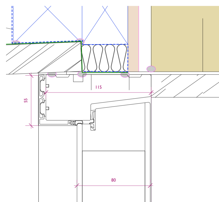
HEAD
