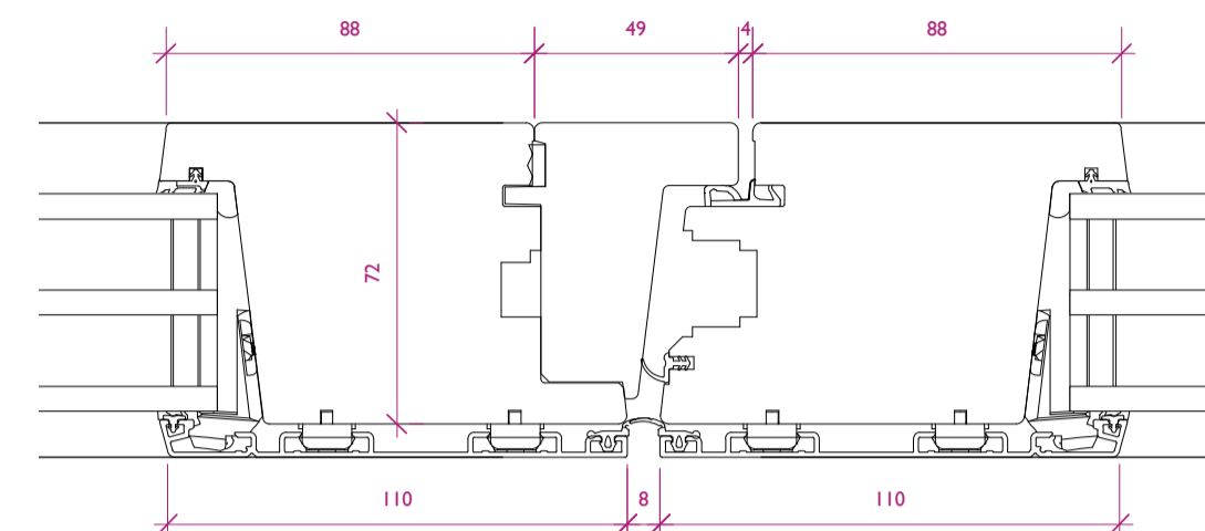
MEETING STILES
