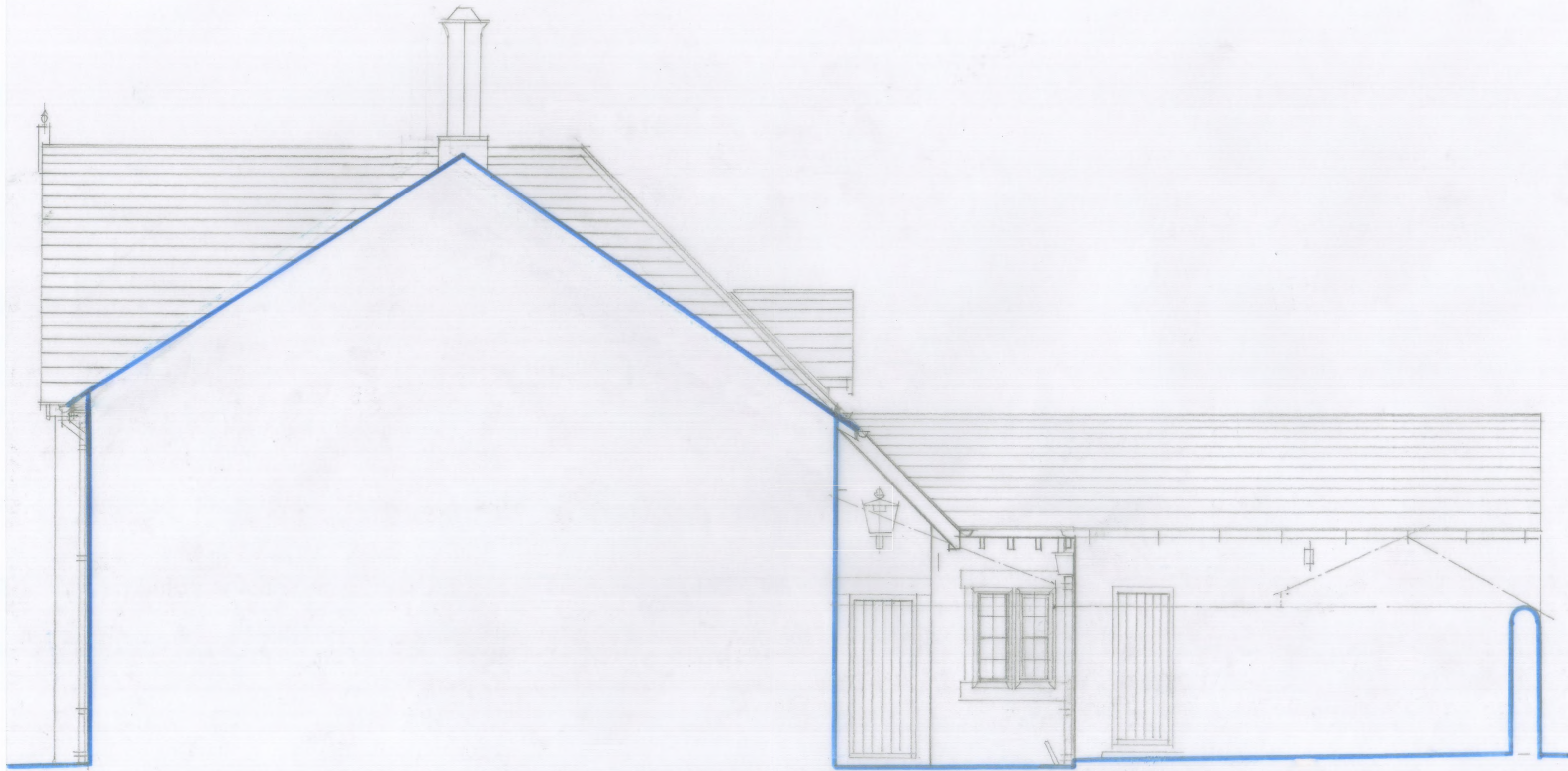
Existing Sectional Side Elevation Scale 1:50
