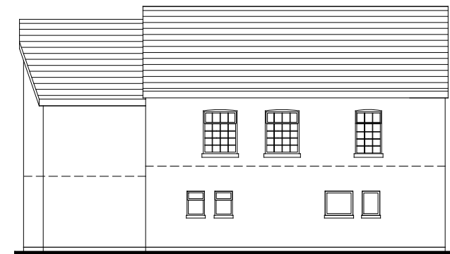
existing east elevation
