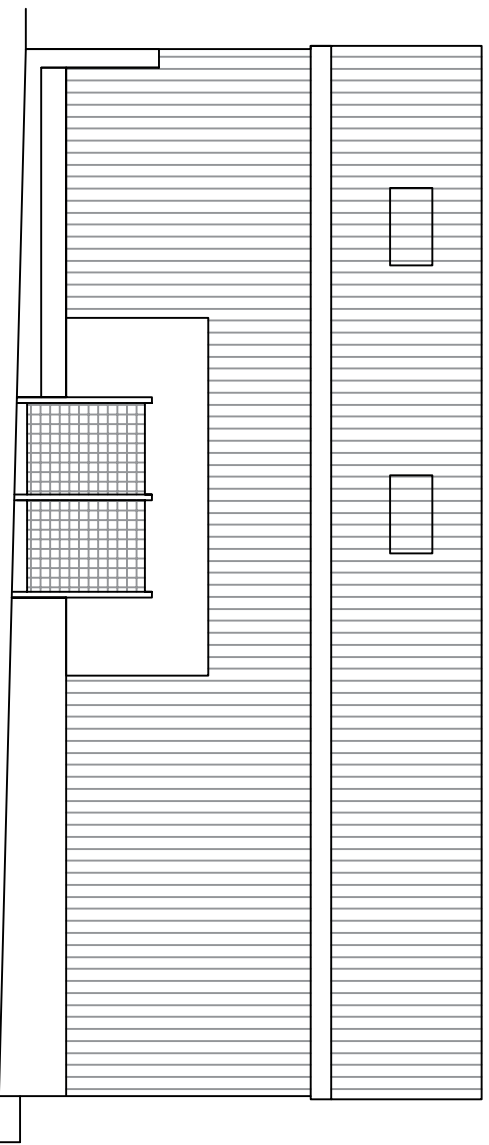
EXISTING NORTH ELEVATION 1:100
